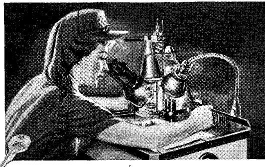
Drilling Diesel Fuel Injector Holes — \frac{6}{1000} th Inch in Diameter—Fuel is forced into the combustion chamber of a Diesel engine through tiny holes. To drill them—GM production experts have developed this highly sensitive machine that insures precision work.
